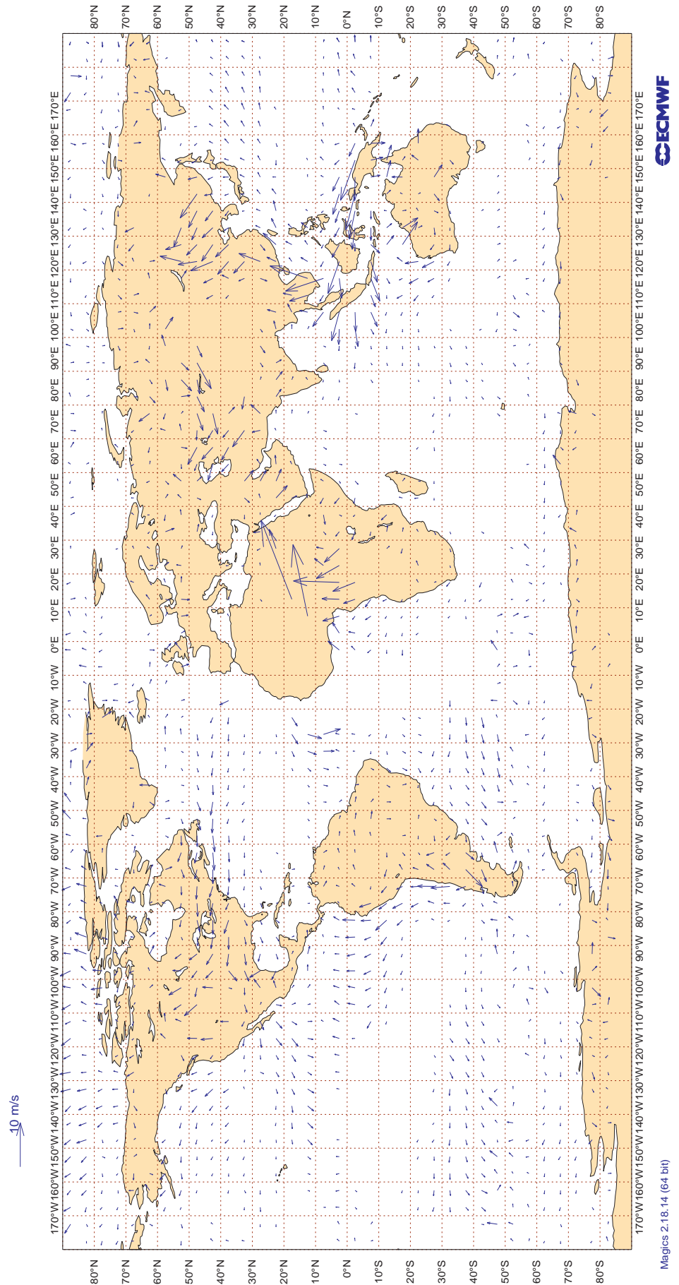
Figure 16 ECMWF Monitoring Statistics: Dec 2013 AMV Winds: 700-1000hPa Wind bias: Observation - FG
