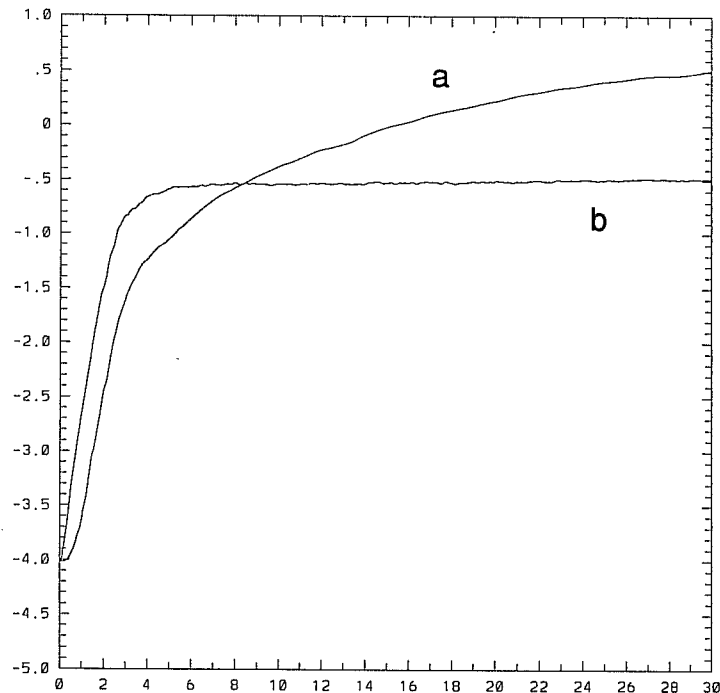
Fig. 4 Variations of \log_{10} E (scale at left) with prediction range \tau (scale, in days, at bottom), shown separately for large scales (variables X_k , curve a) and small scales (variables Y_{j,k} , curve b), for 30 days, as determined by 25 pairs of integrations of Eqs. (2) and (3), with the parameter values of Fig. 3.
