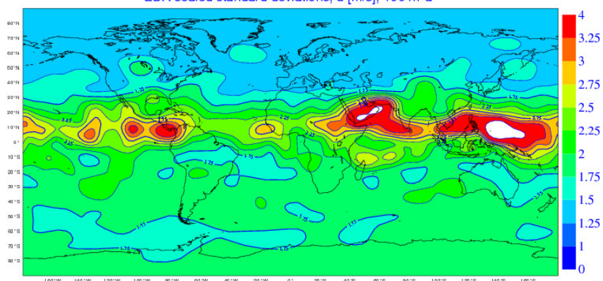
EDA scaled standard deviations, u [m/s], 250 hPa
