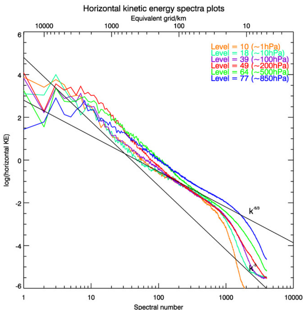
Horizontal kinetic energy power spectrum for T3999 (~5 km) at various model levels
