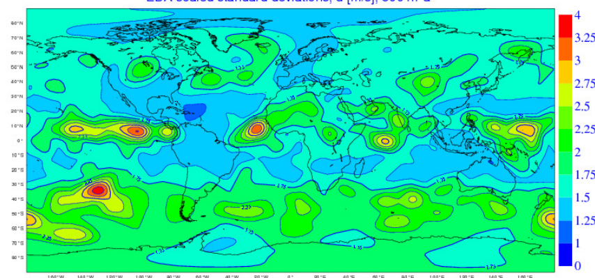
EDA scaled standard deviations, u [m/s], 500 hPa
