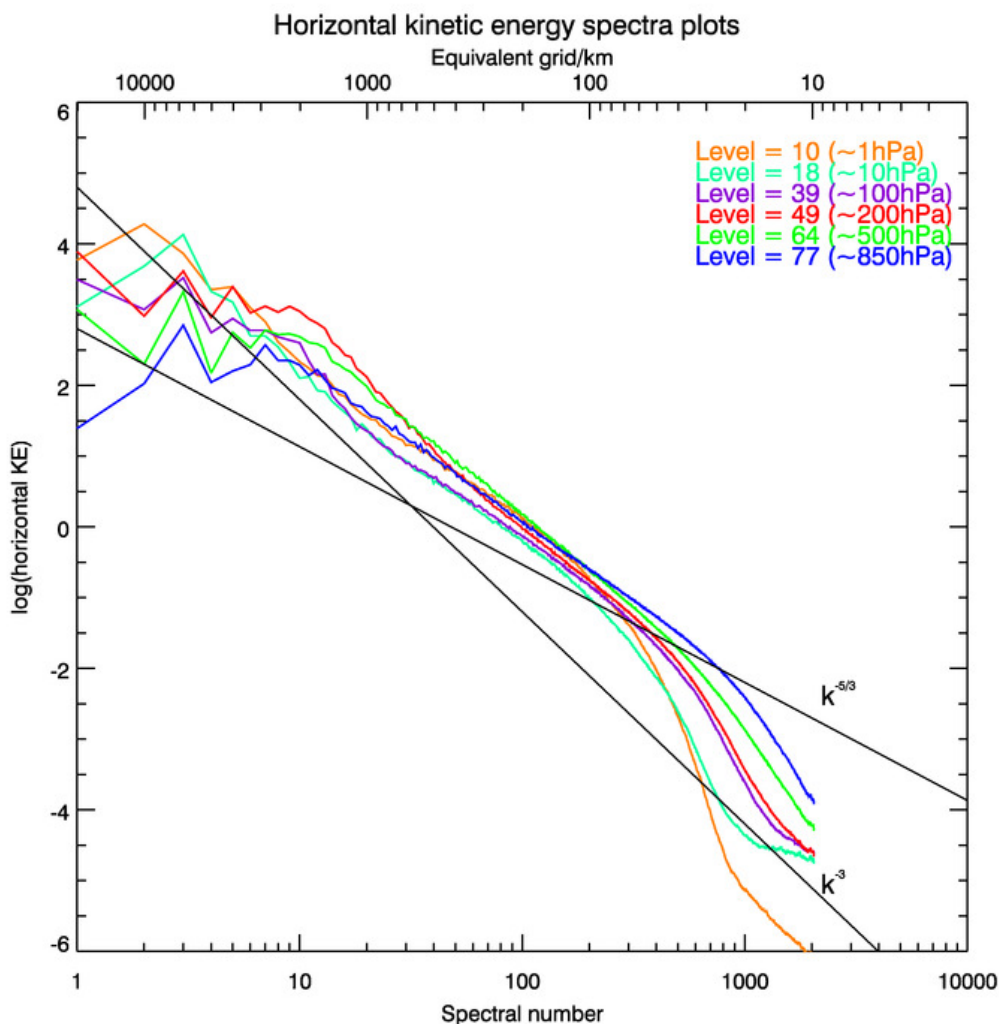
Horizontal kinetic energy power spectrum for T2047 (~10 km) at various model levels.
