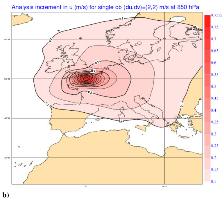
Map of analysis increments in u at 850 hPa from a single wind vector assimilated at a) the end of the 4D-Var window (plot valid at end of time window) b) start of the time window (plot valid at start of time window)
