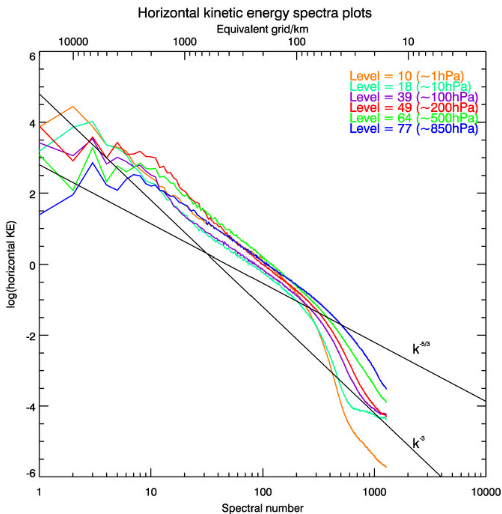
Horizontal kinetic energy power spectrum from the operational T1279 (~16 km) at various model levels
