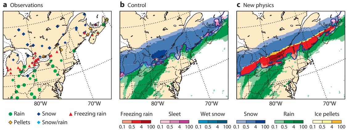
Figure 6 A significant freezing rain event over eastern North America on 22 December 2013. (a) Observations from SYNOP and METAR reports of precipitation type at 06 and 12 UTC. Precipitation rate and type from the 9-hour forecast from the 00 UTC analysis on 22 December 2013 using (b) the current operational model as the control and (c) the model with the new physics. Shading in (b) and (c) is for 0.1, 0.5 and 4 mm hr -1 and the thick blue contour is the 2-metre 0°C isotherm.
