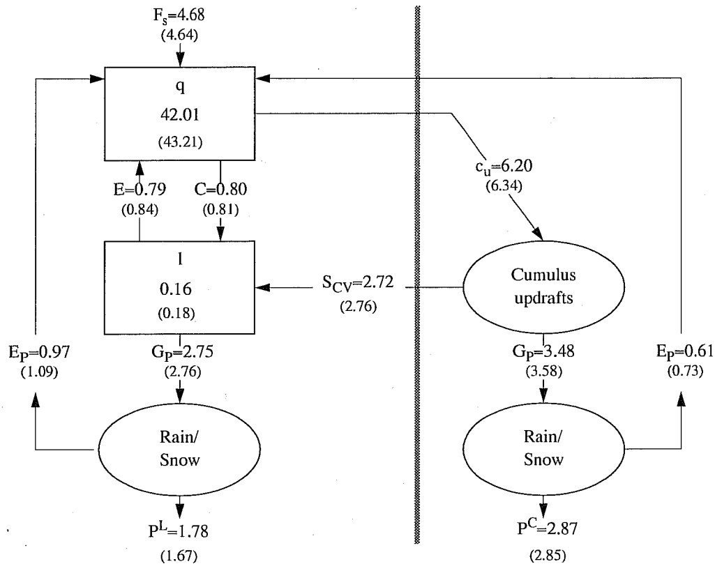
Figure 10: Hydrological cycle: Tropical average ( 20^\circ N to 20^\circ S ) of atmospheric water vapour q , cloud liquid water/ice content l , and conversions between water vapour, cloud water/ice and rain/snow in stratiform clouds (left) and cumulus updrafts (right). The results are averages over a 30 day integration at T63L31 initialized on 1 July 1998 with the new scheme with values for the control model shown in parantheses. Units are mm for water reservoirs and mm/day for conversion terms. The terms are: F_s - surface evaporation, C - large-scale condensation of cloud liquid/ice, E - large-scale evaporation of cloud liquid water/ice, S_{CV} - source of cloud liquid water/ice from convection, G_P - generation of precipitation, E_P - evaporation of precipitation, c_u - condensation in cumulus updrafts, P^L - large-scale precipitation at the surface, P^C - convective precipitation at the surface.
