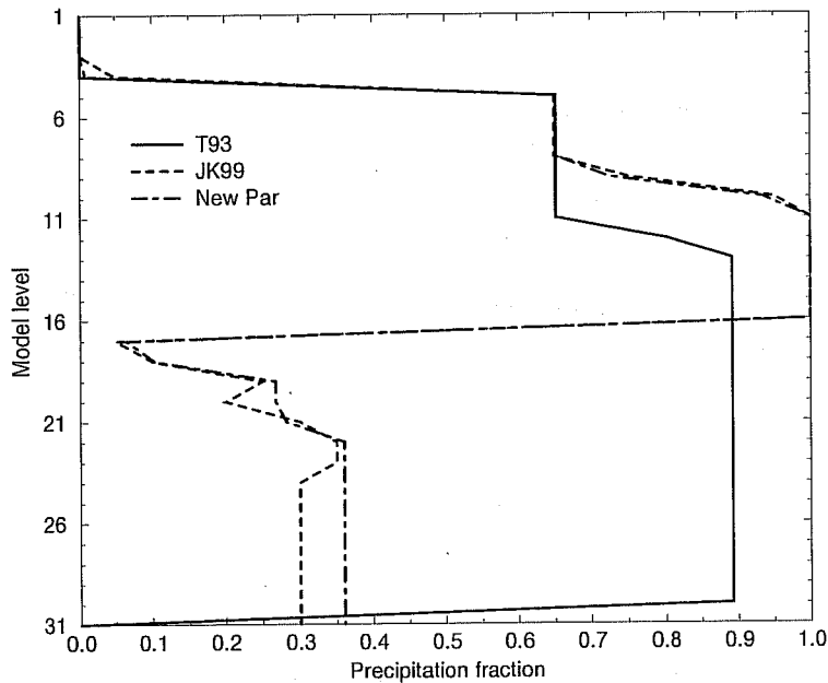
Figure 3: Precipitation fraction at a single tropical point as predicted in a single time step by the T93 parametrization (solid), the JK99 sub-grid model (dashed) and the new parametrization (dot-dashed).
