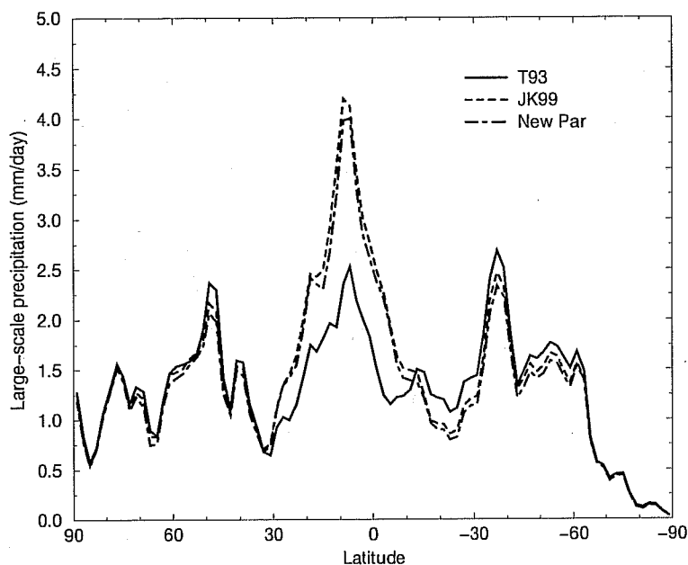
Figure 7: Zonal mean large-scale precipitation as predicted in a single time step by the T93 parametrization (solid), the JK99 sub-grid model (dashed) and the new parametrization (dot-dashed).
