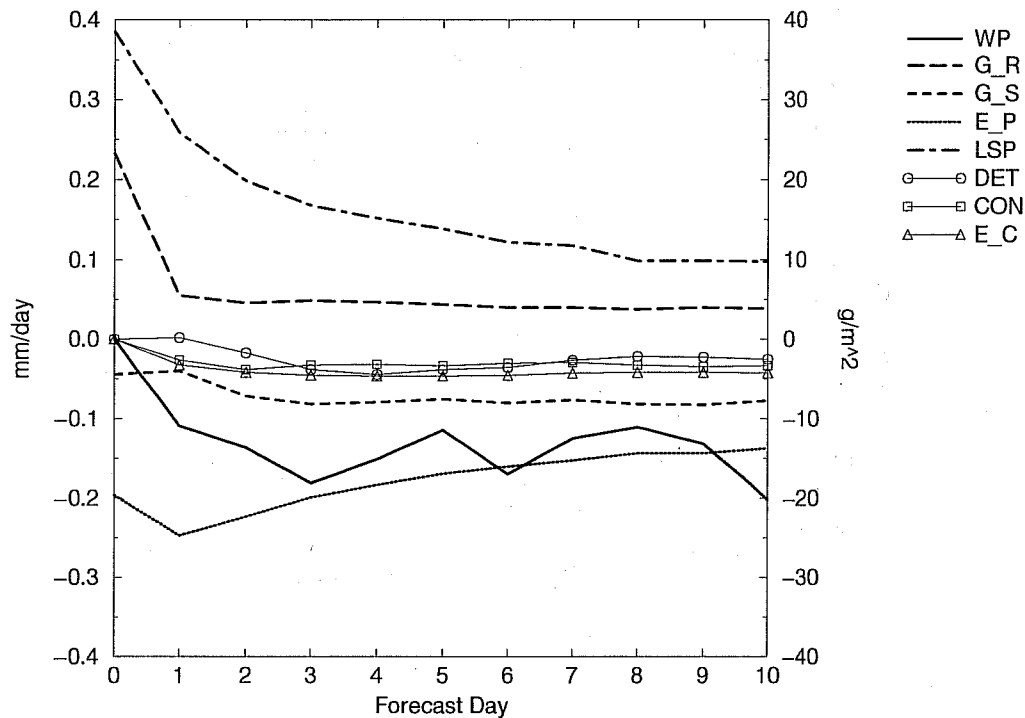
Figure 11: Hydrological cycle: Time series of the difference (New Par - T93) in the tropical average ( 20^{\circ}N to 20^{\circ}S ) of some terms shown in Figure 10 for the first 10 forecast days. Day 0 represents the first model time step. The terms are: WP - liquid+ice water path, G_R - generation of rain, G_S - generation of snow, E_P - evaporation of large-scale precipitation, LSP - large-scale precipitation at the surface, DET - source of cloud liquid water/ice from convective detrainment, CON - large-scale condensation of cloud liquid water/ice, E_C - large-scale evaporation of cloud liquid water/ice.
