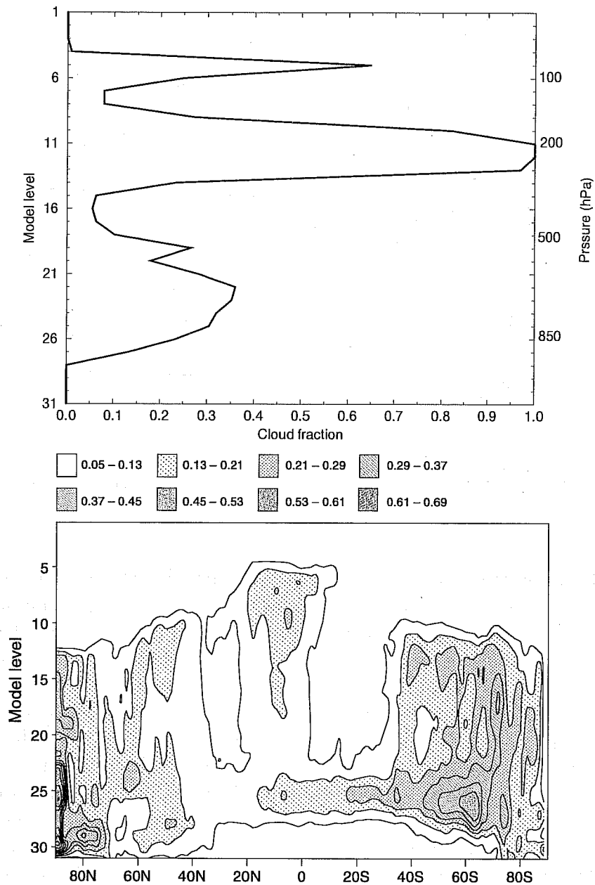
Figure 2: Initial cloud fraction distribution for the single time step experiments for the single column model (top) and the global model (bottom).
