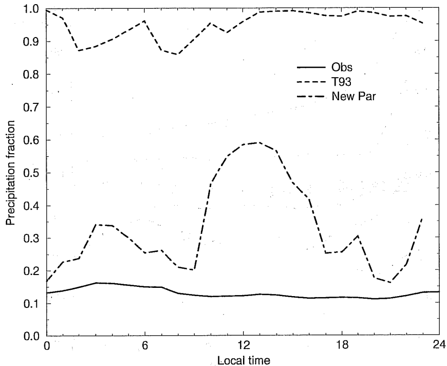
Figure 12: Monthly average stratiform (i.e. Large-scale) precipitation fraction at the surface as a function of local time. Shown are observations by ship-borne radar during TOGA/COARE (solid) and predictions for December 1992 at 2^{\circ}S and 155^{\circ}E by a T63L31 integration using the T93 scheme (dashed) and the new parametrization (dot-dashed).
