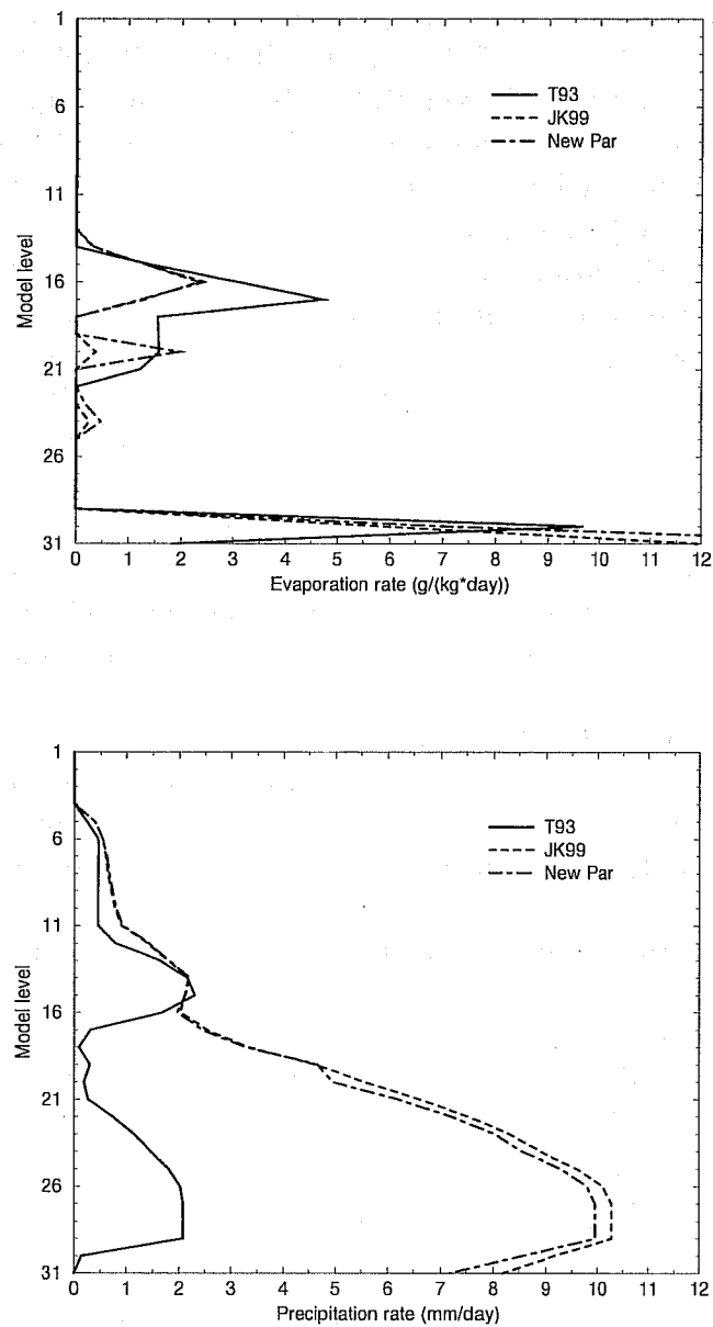
Figure 4: Grid-mean evaporation rate (top) and precipitation rate (bottom) as predicted in a single time step by the T93 parametrization (solid), the JK99 sub-grid model (dashed) and the new parametrization (dot-dashed).
