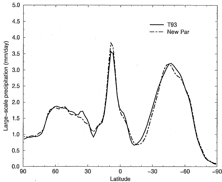
Figure 8: Zonal mean large-scale precipitation for JJA87 from an ensemble of three integrations using the current (solid) and new (dot-dashed) precipitation schemes
