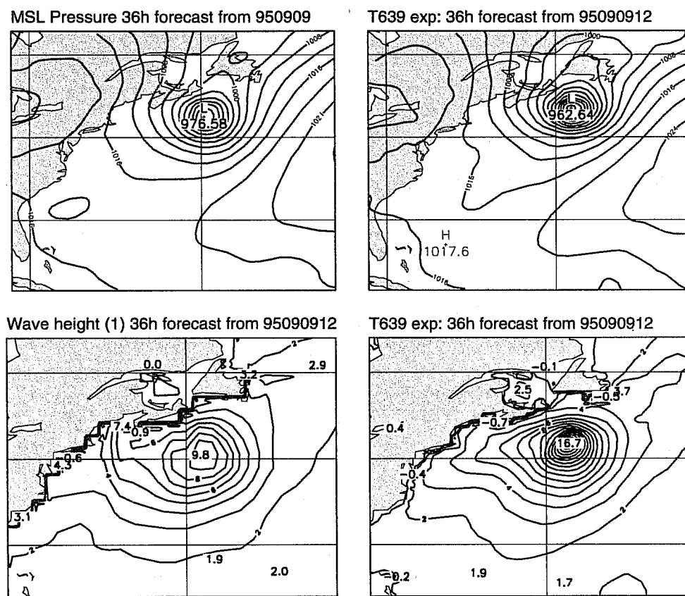
Figure 1: Progress in extreme sea state forecasting due to increase in spatial resolution as illustrated by the 36 hour forecast of Hurricane Luis. The top left panel shows the operational forecast mean sea level pressure of 1995090912 UT with T213 resolution while the top right panel shows the 36 hr forecast with T639 resolution. The bottom panels show the corresponding 36hr wave height forecast forced by low(left) and high(right) resolution winds.
