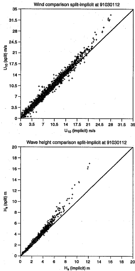
Figure 7: Comparison of surface winds (panel a) obtained from the split scheme and implicit scheme. The consequences for significant wave height are shown in panel b).
