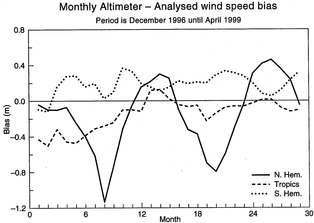
Figure 11: Monthly mean difference between Altimeter wind speed and analysed wind speed over the period of December 1996 until April 1999. Areas are Northern Hemisphere, Tropics and the Southern Hemisphere.
