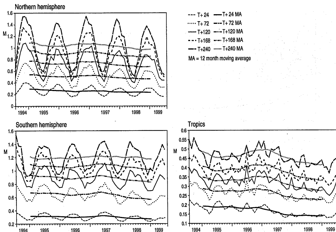
Figure 4: Standard deviation of wave height error (forecast versus analysis) for Northern Hemisphere, Southern Hemisphere and Tropics over the period of August 1994 until July 1999.
