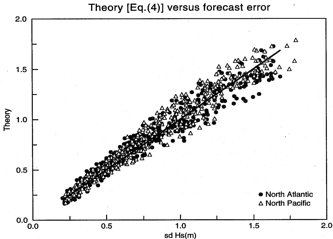
Figure 6: Comparison of random wave height error obtained from the theory(Eq.(4)) with the actual forecast error from the ECMWF archives for the North Atlantic and the North Pacific.
