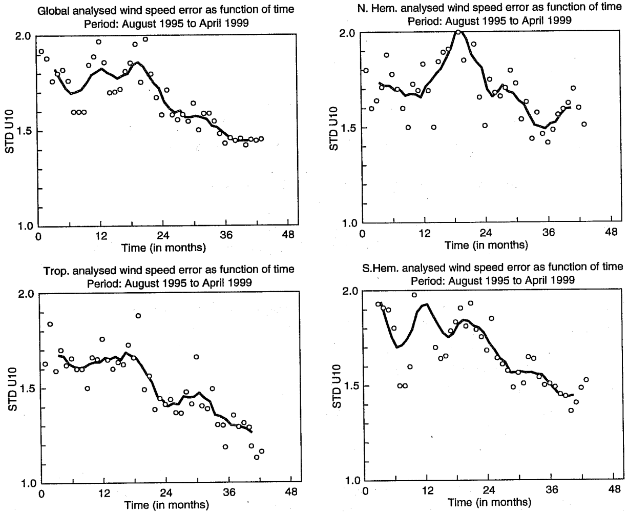
Figure 12: Standard deviation of analysed wind speed error as obtained from the comparison between wind speed analysis and ERS-2 Altimeter winds over the period August 1995 to April 1999. Areas are the whole Globe (oceans only), Northern Hemisphere, Southern Hemisphere and Tropics. The open circles are monthly data while the full line is a 6 month running average.
