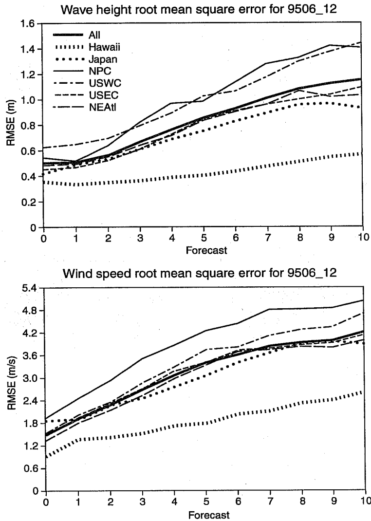
Figure 2: Evolution of rms error for wave height(top) and wind speed(bottom) as a function of forecast day at buoy locations. Symbols refer to different areas as displayed in the legend.
