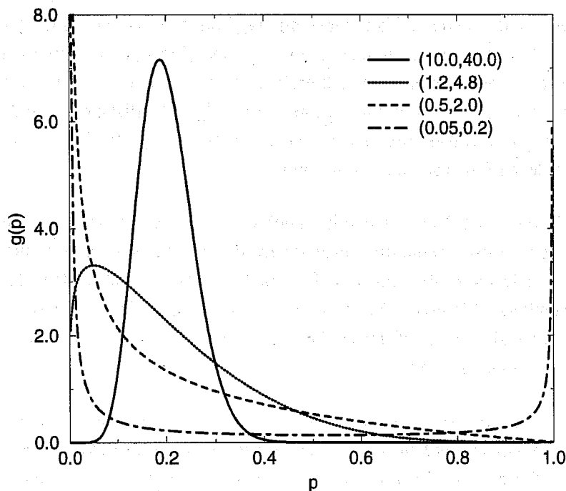
Figure 2: Examples of the beta distribution for different choices of the distribution parameters r and s . The mean is the same for all cases
