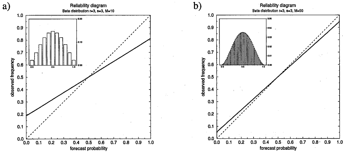
Figure 3: Reliability diagrams for theoretical ensemble forecasts for (a) 10-member EPS; (b) 50-member EPS. Distribution of underlying forecast probabilities is completely reliable and specified by beta distribution with r = s = 3 .
