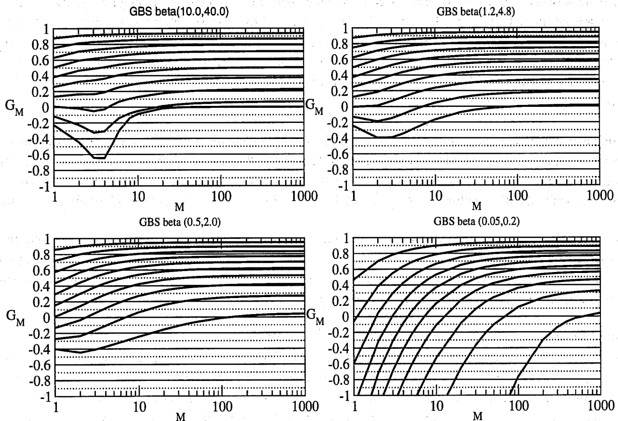
Figure 8: The variation of a generalised skill score G_M with ensemble size for four different distributions of users, specified by the four beta functions shown in Fig. 2. The 10 curves in each panel correspond to the curves for B_M in Fig. 1. Note that the horizontal scale has been extended to allow for the greater sensitivity to ensemble size.
