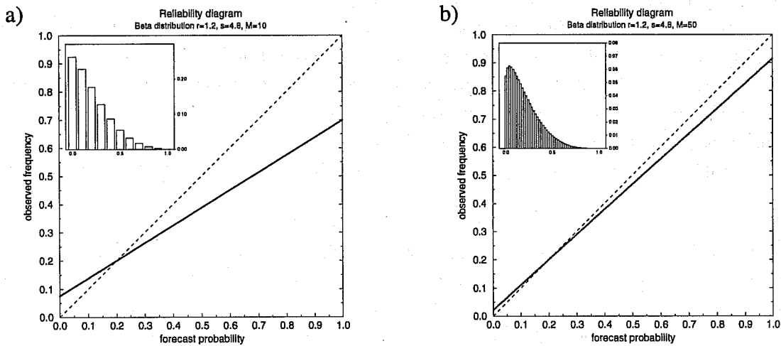
Figure 4: Reliability diagrams for theoretical ensemble forecasts for (a) 10-member EPS; (b) 50-member EPS. Distribution of underlying forecast probabilities is completely reliable and specified by beta distribution with r=1.2, s=4.8 .
