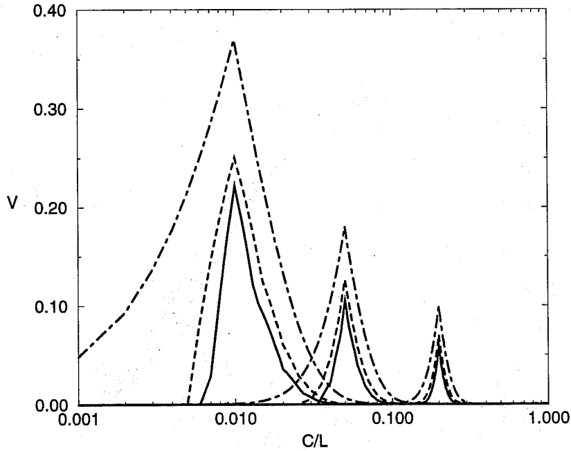
Figure 7: As Fig. 6 but for B_\infty = 0.01 .
