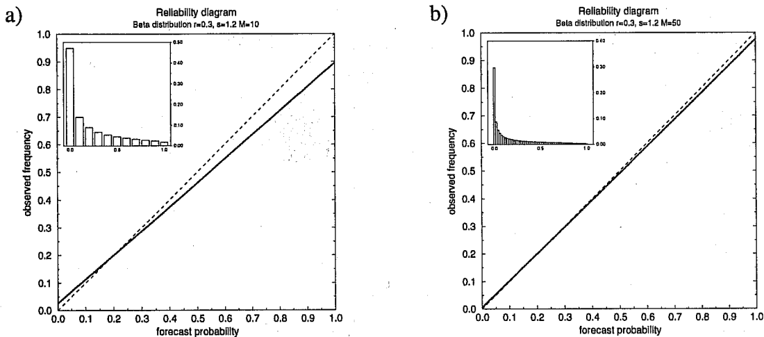
Figure 5: Reliability diagrams for theoretical ensemble forecasts for (a) 10-member EPS; (b) 50-member EPS. Distribution of underlying forecast probabilities is completely reliable and specified by beta distribution with r=0.3 , s=1.2 .
