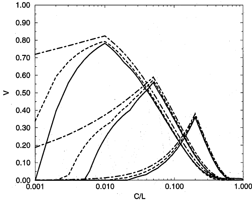
Figure 6: Relative value as a function of cost-loss ratio for three events: \bar{o} = 0.01 (left-most set of curves); \bar{o} = 0.05 (centre); and \bar{o} = 0.2 (right-most curves). The Brier skill score for the underlying forecasts is the same for each event, B_{\infty} = 1/7 . The three curves in each set are for 50-member EPS (solid), 100-member EPS (dashed) and the potential value of the underlying distribution (limit for large ensemble, dash-dotted curve).
