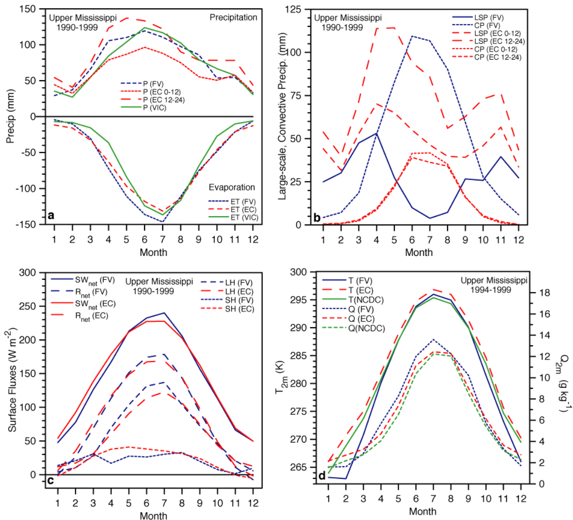
Figure 6 As Figure 4 for Upper Mississippi river basin.
