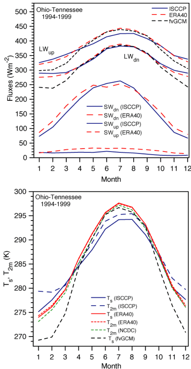
Figure 10 As Figure 9 for Ohio-Tennessee basin.
