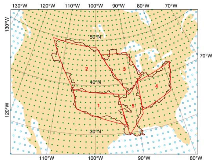
Figure 1 River basin budgets in ERA-40 for the Mississippi
