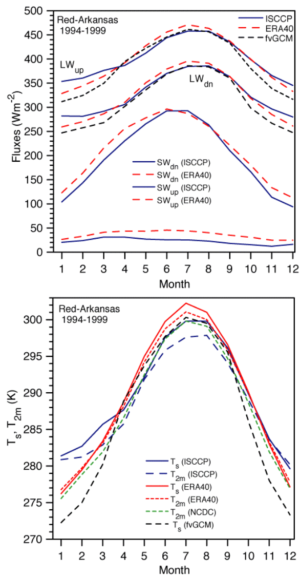
Figure 9 Comparison of surface radiation budget components (above) and surface temperatures (below) for Red-Arkansas basin.
