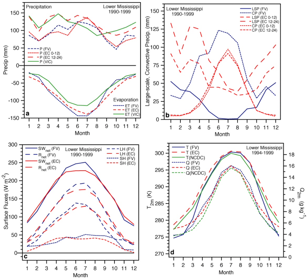
Figure 8 As Figure 4 for Lower Mississippi river basin.
