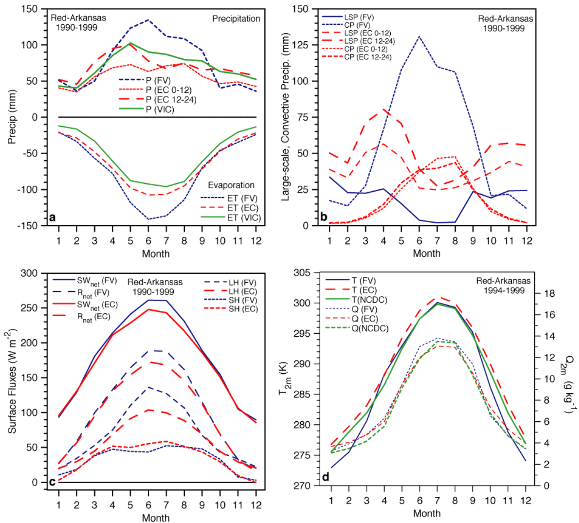
Figure 4 a) Precipitation and evaporation for ERA-40, fvGCM climate and observations, b) Large-scale and convective scale precipitation, c) Fluxes in energy budget, d) 2-m temperature and specific humidity.
