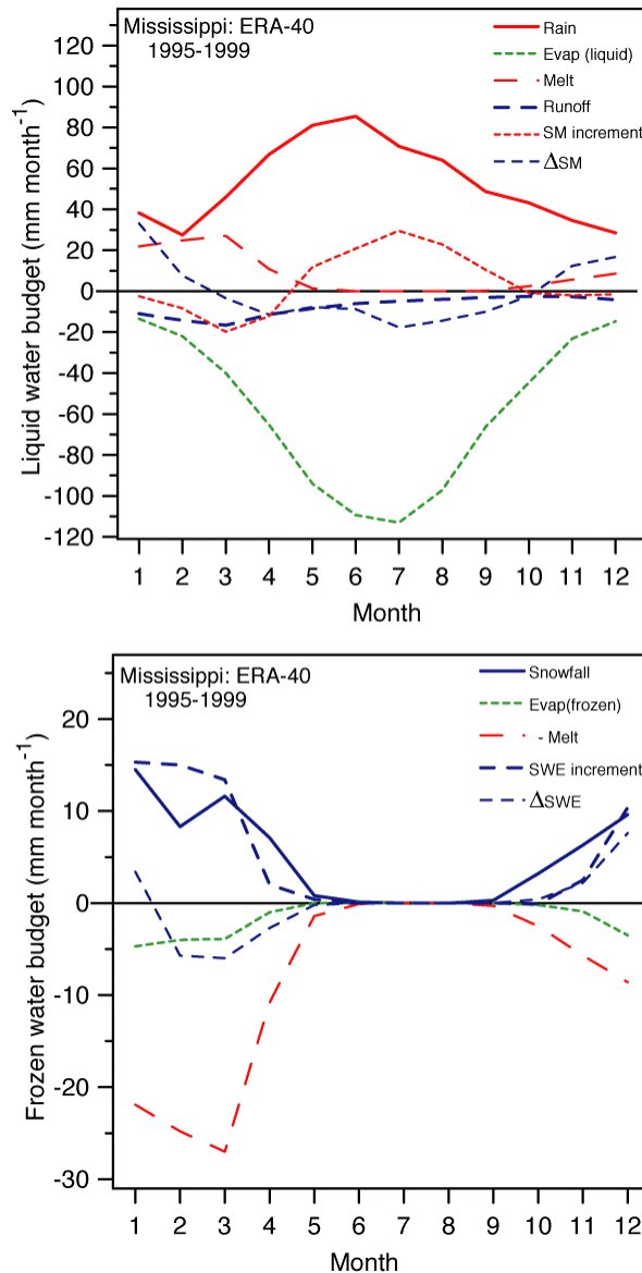
Figure 3 Mean annual cycle of liquid and frozen water budgets for ERA-40 for 1995-1999.
