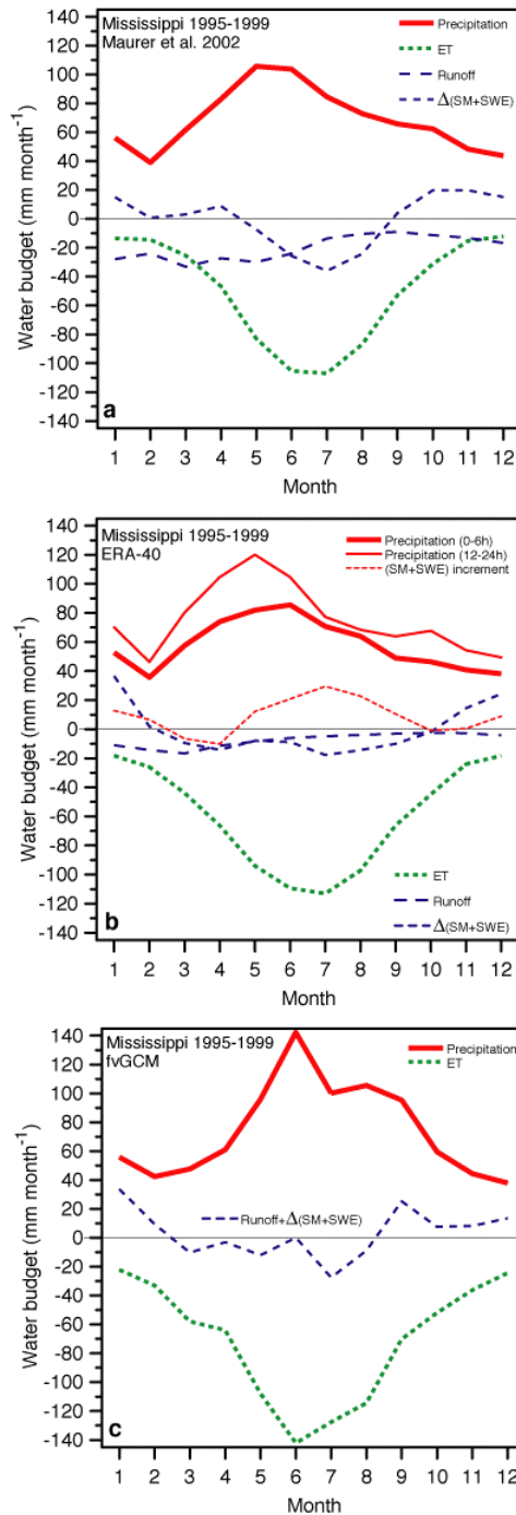
Figure 2 Water budget annual cycle for the Mississippi basin from Maurer et al. [2002], ERA-40, and fvGCM for 1995-1999.
