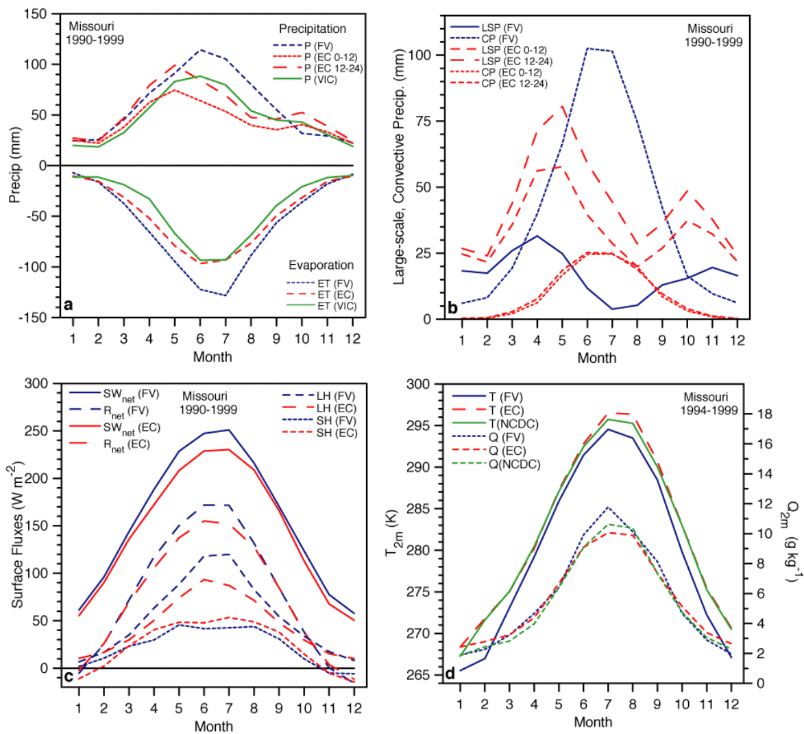
Figure 5 As Figure 4 for Missouri river basin.
