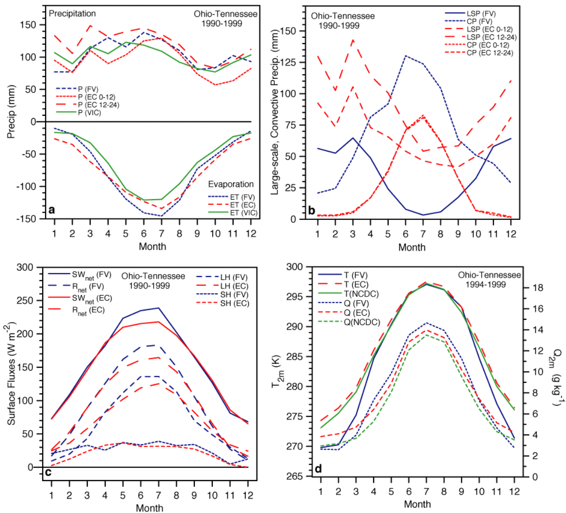
Figure 7 As Figure 4 for Ohio-Tennessee river basin.
